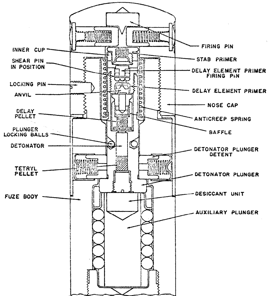
Fig 1-22 BASE FUZE Mk21 (ASSEMBLED POSITION)
